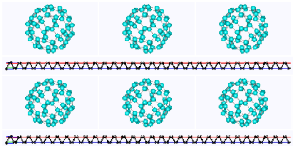
Fig. 2. Polymer chain with diffusing polaron surrounded with rotating fullerene molecules
