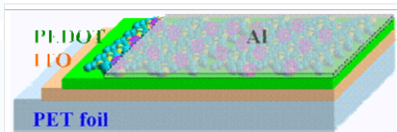
Fig. 1. The scheme of plastic solar cells. PET - PolyEthyleneTerephtalate, ITO - Indium Tin Oxide, PEDOT - Poly(3,4-EthyleneDiOxyThiophene), Al - Aluminium.]]
